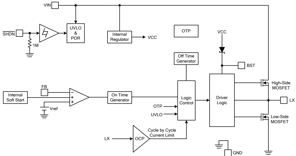
Figure 4. Block Diagram of FR9204FH
