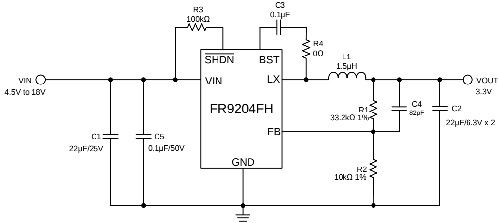
Figure 2. FR9204FHS9 Application Circuit
