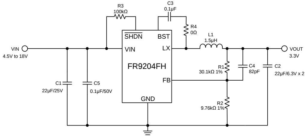
Figure 3. FR9204FHSD Application Circuit
