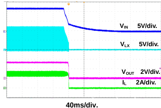
Figure 16. Power Off Through VIN Waveform
