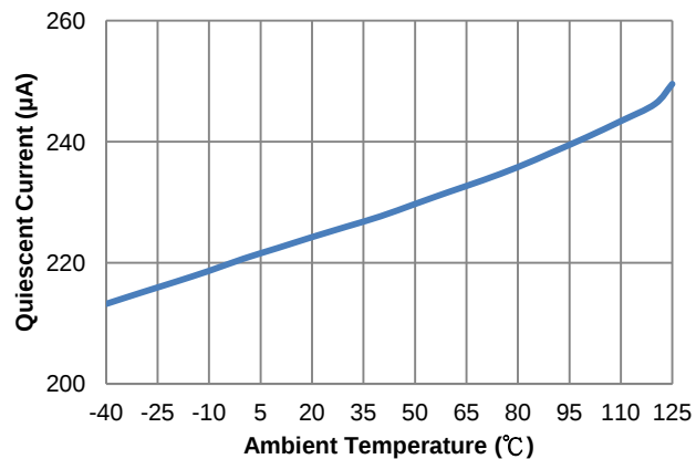
Figure 9. Quiescent Current vs. Ambient Temperature
