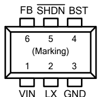
Figure 1. Pin Assignments of FR9204FH
