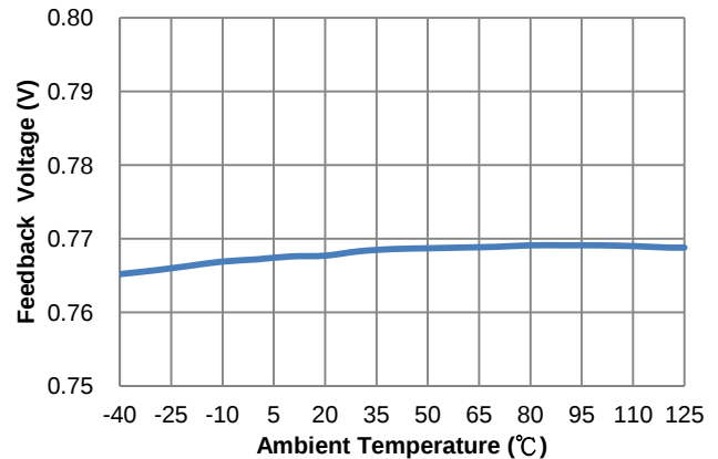
Figure 10. Feedback Voltage vs. Ambient Temperature
