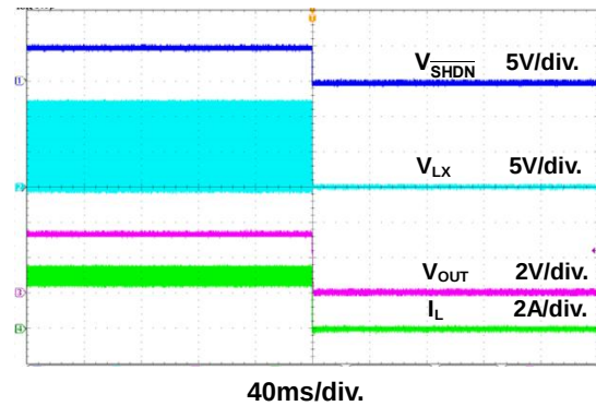
Figure 20. Power Off Through \overline{SHDN} Waveform
