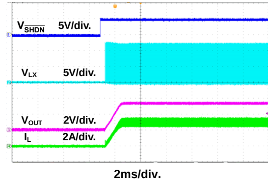
Figure 18. Power On Through \overline{SHDN} Waveform
