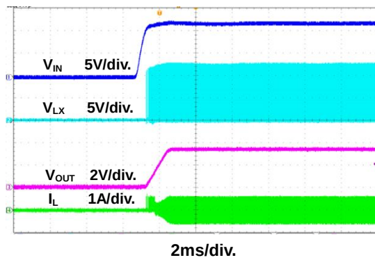
Figure 13. Power On Through VIN Waveform
